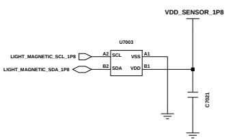
MAGNETIC SENSOR
