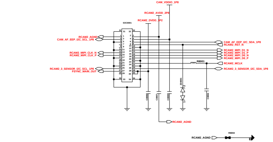
RCAM2_5M_UW (30pin)_GC5035 COPY FROM SM-A12_LTE
