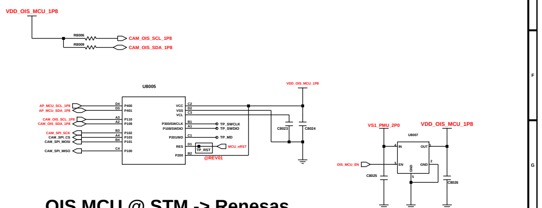
OIS MCU @ STM -> Renesas
