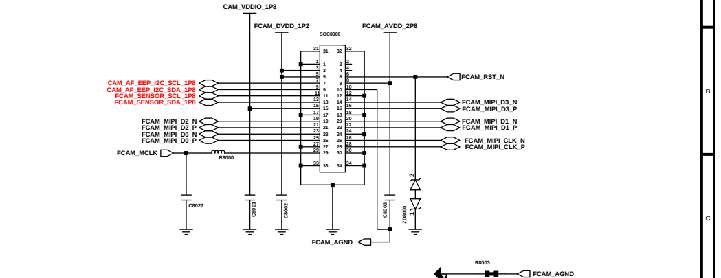
FRONT_13M CAMERA (NEW - IMX258)
