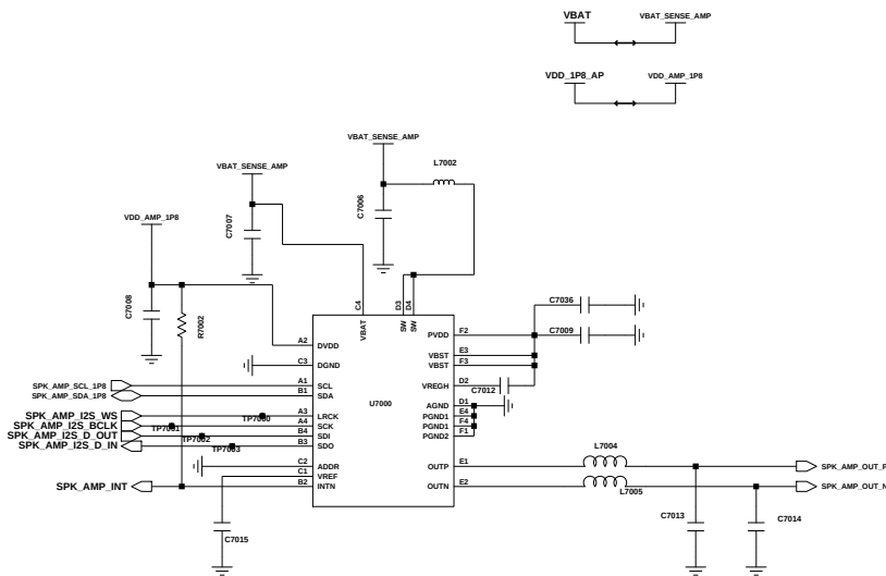
SPK AMP
