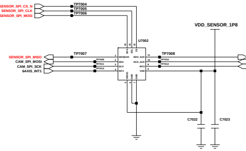
ACC&GYRO SENSOR
