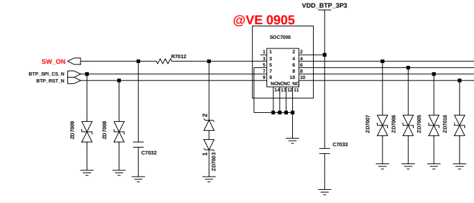
PWR & SIDE FPS
