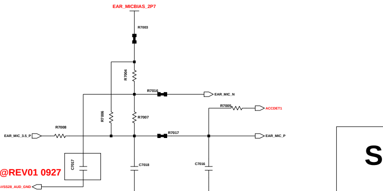
EAR MIC
