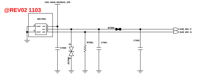
2nd MIC
