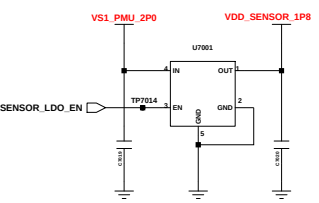
SENSOR LDO
