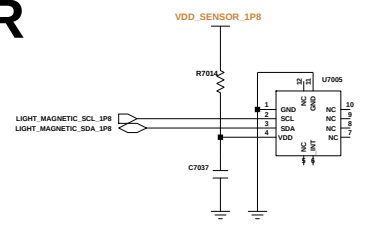
AMBIENT SENSOR
